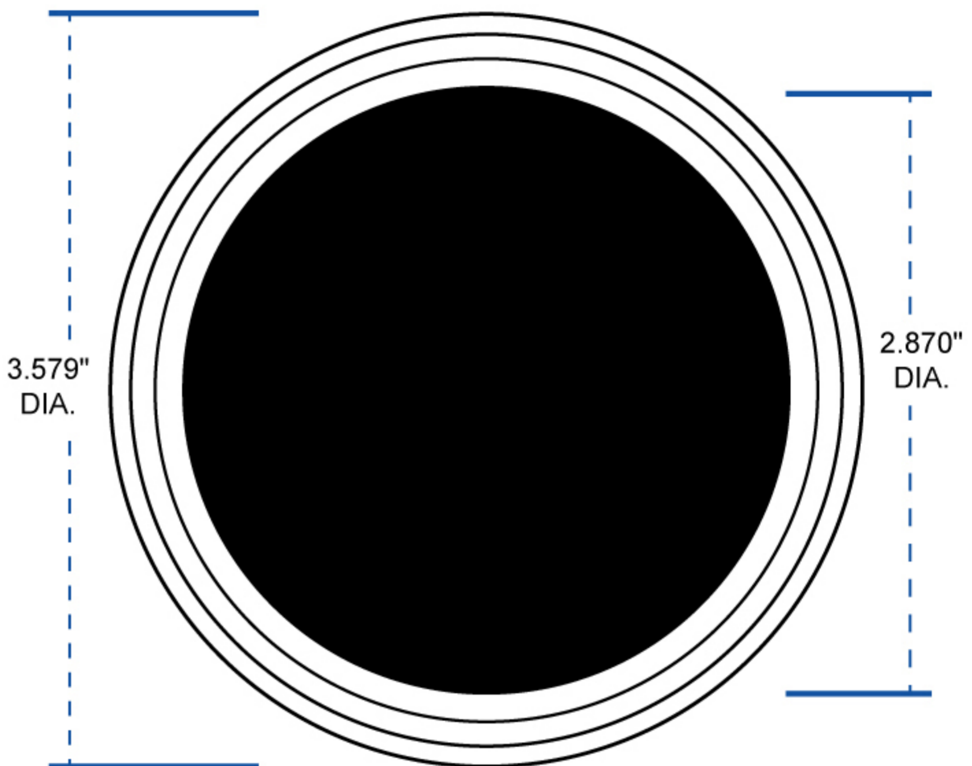
3" Clamp
