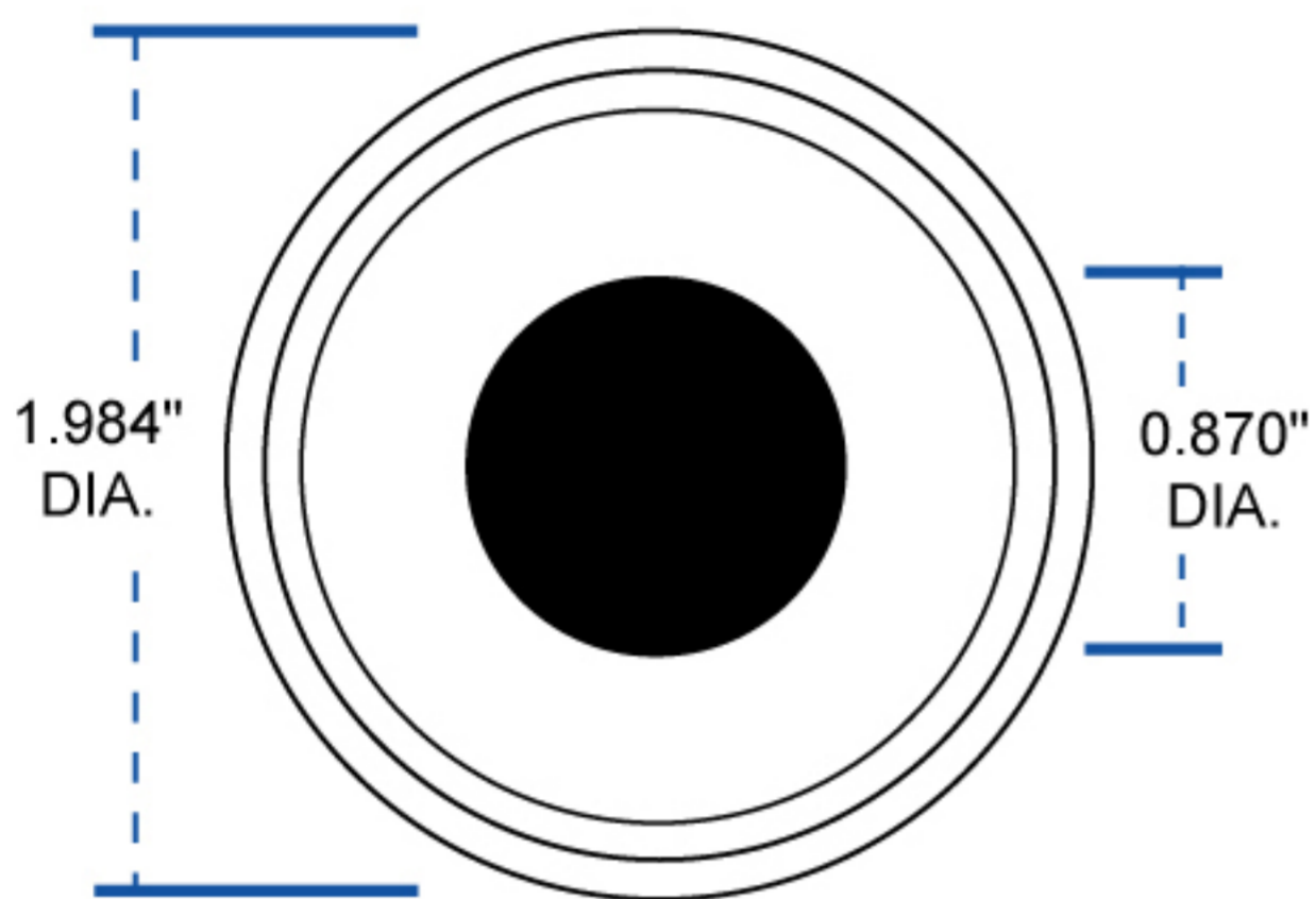
1" Clamp
